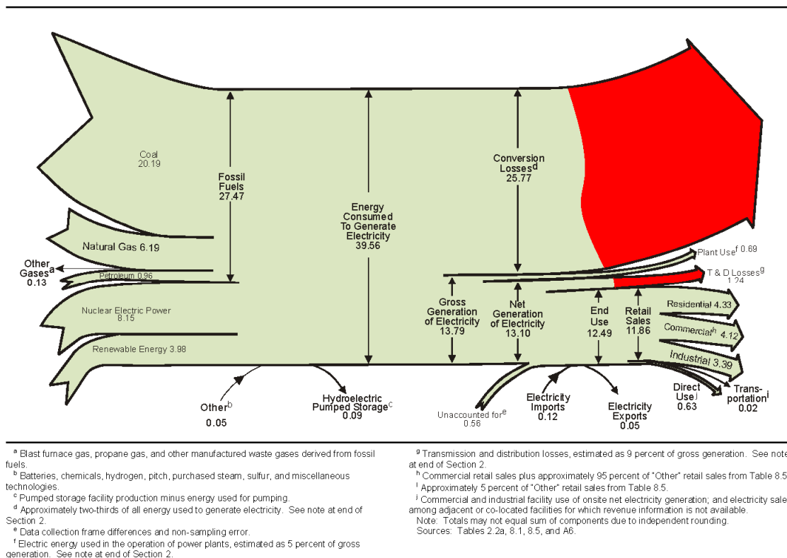
Diagram 14.1. Electricity Flow, 2002 (Quadrillion BTU – Quads). From Annual Energy Review 2002, 2003, Energy Information Administration, U.S. Department Of Energy. http://www.eia.doe.gov/emeu/aer/ , p. 219. Wasted energy is shown in red. (Red color added by J. Rothwell.)
