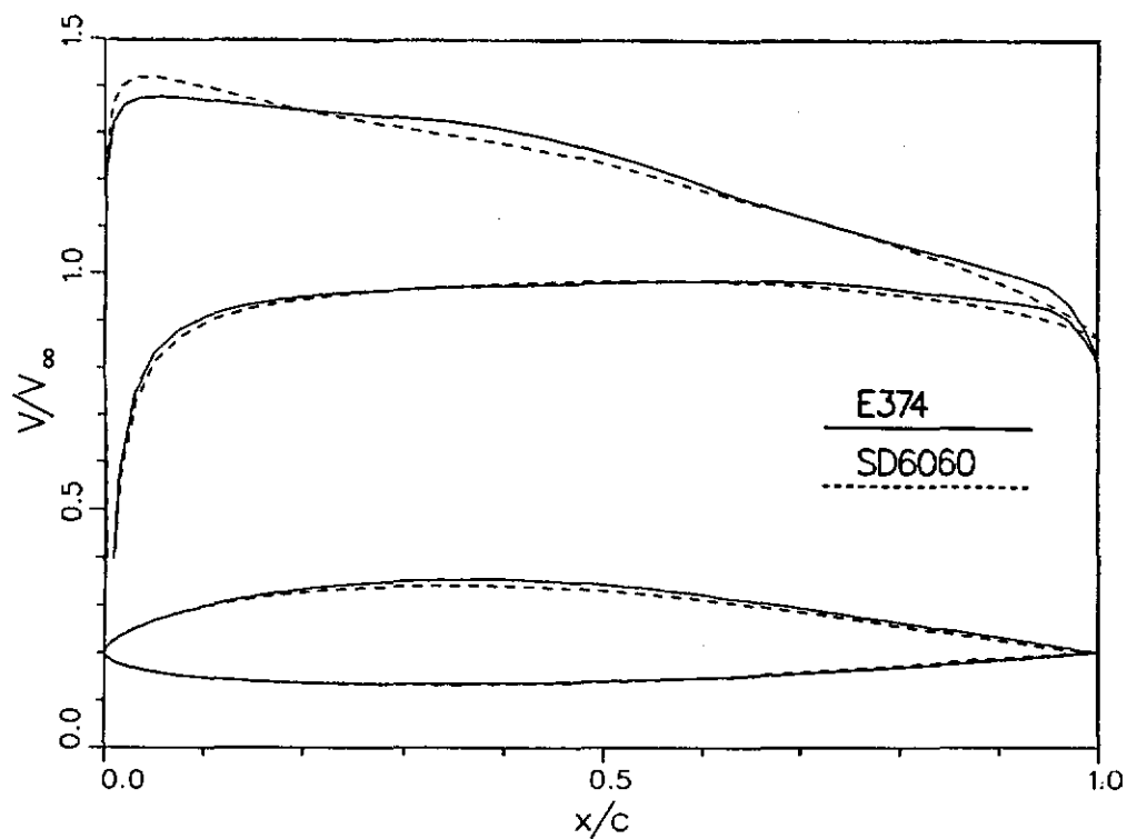
Fig. 4.1 Inviscid velocity distributions: \alpha_{w.r.t.0L} = 5^\circ ( C_l = 0.55 ).
