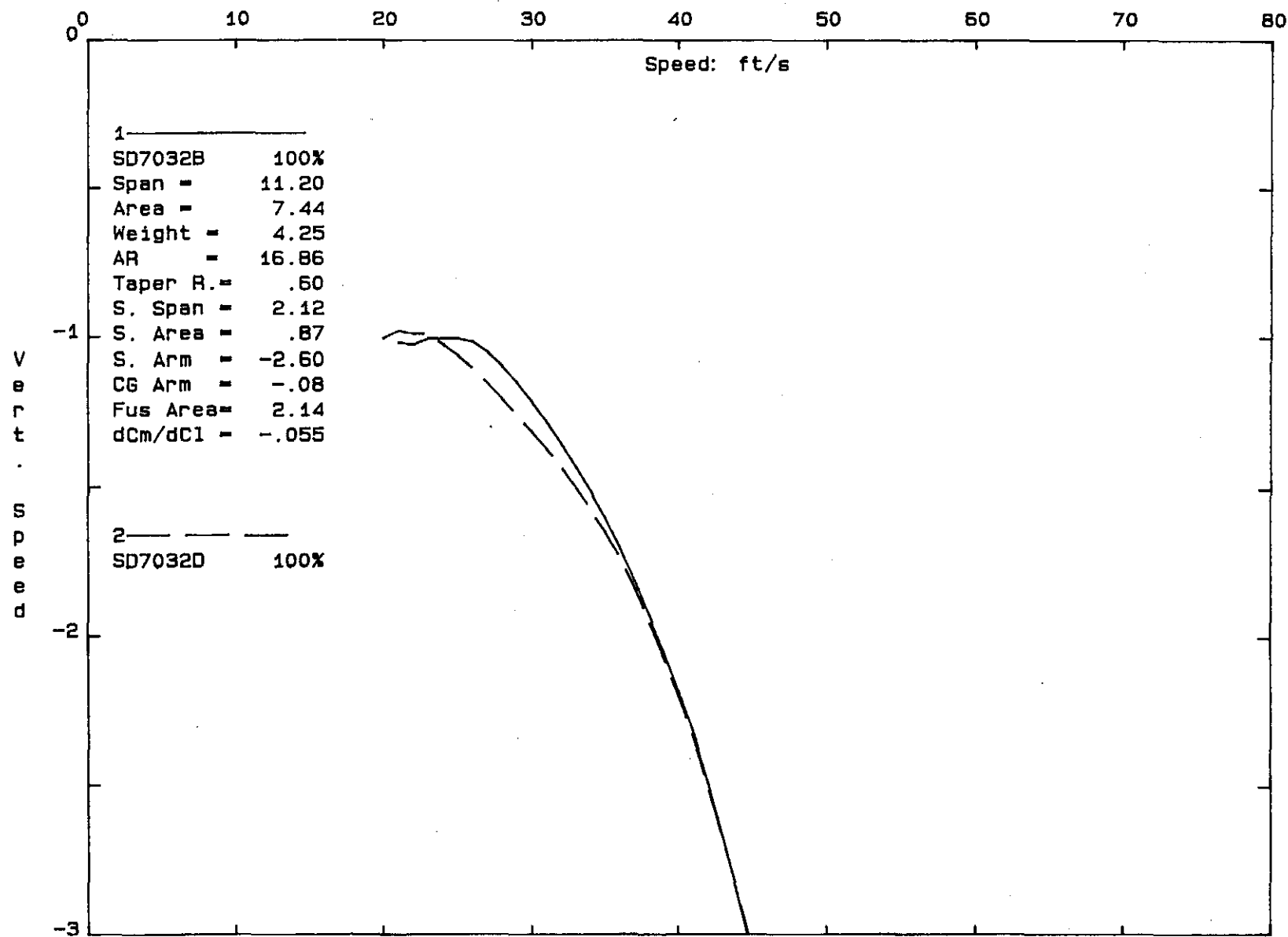
Fig. 5.10 (b) Aircraft Polar: SD7032B-PT vs SD7032D-PT
