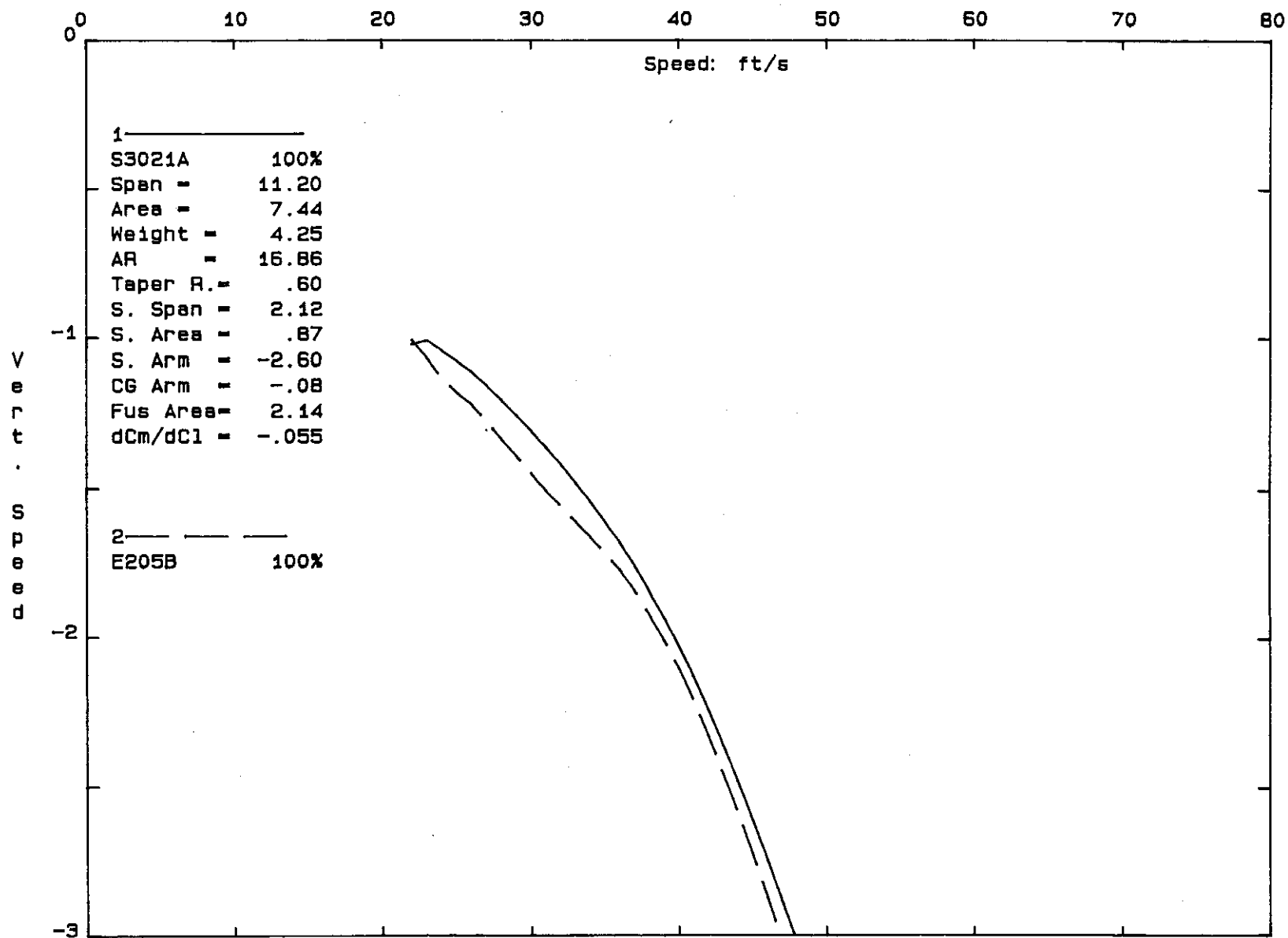
Fig. 5.9 (b) Aircraft Polar: S3021A-PT vs E205B-PT
