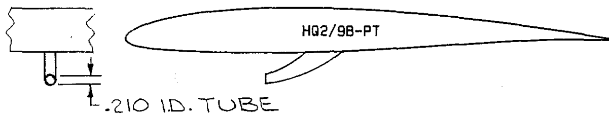
Fig. 5.8 Ram configuration.
