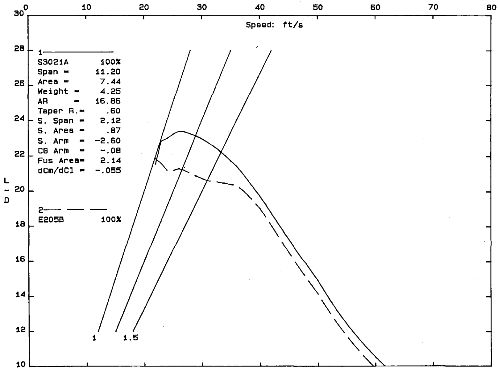
Fig. 5.9 (a) Aircraft Polar: S3021A-PT vs E205B-PT
