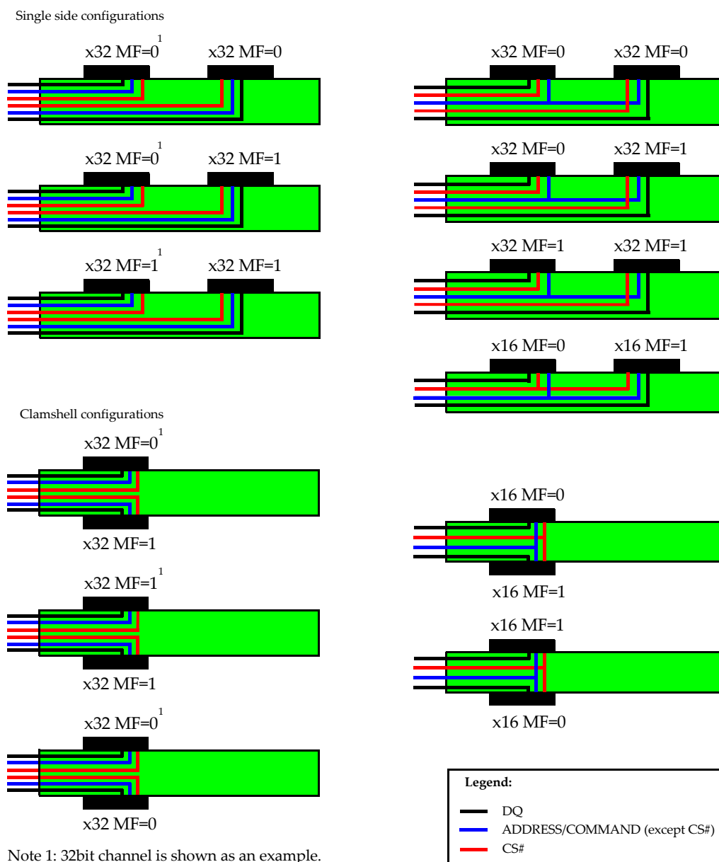
Figure 88. Example GDDR5 PCB Layout Topologies
