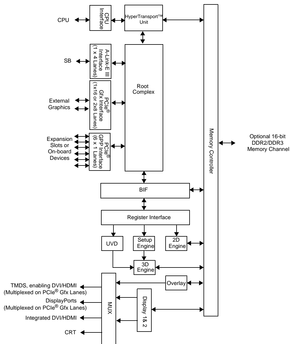
Figure 2-1 RS880D Internal Block Diagram
