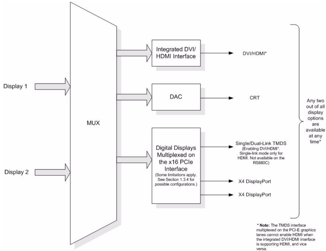
Figure 1-2 RS880D Multiple Display Options
