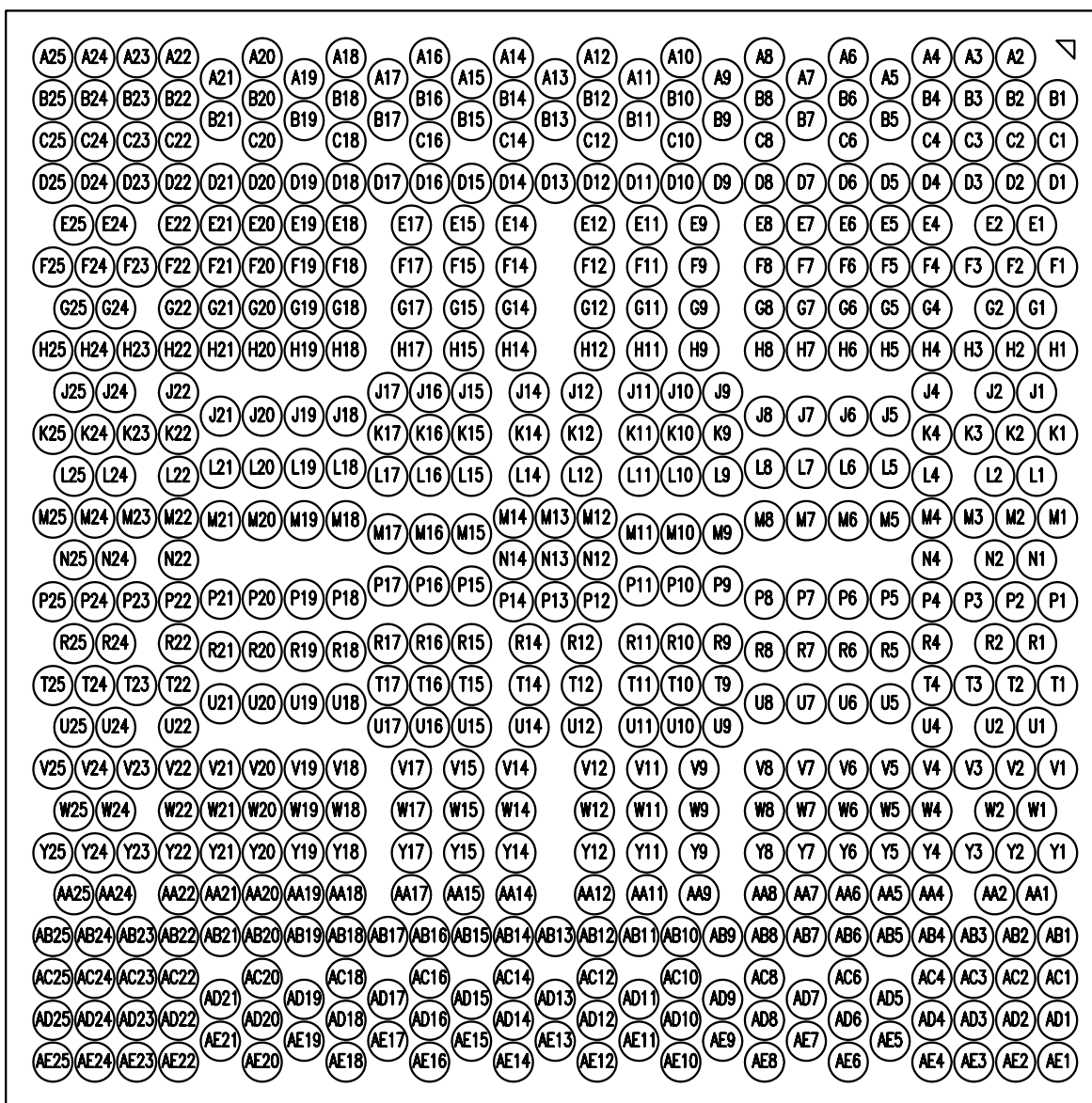
Figure 5-3 RS880D Ball Arrangement (Bottom View)
