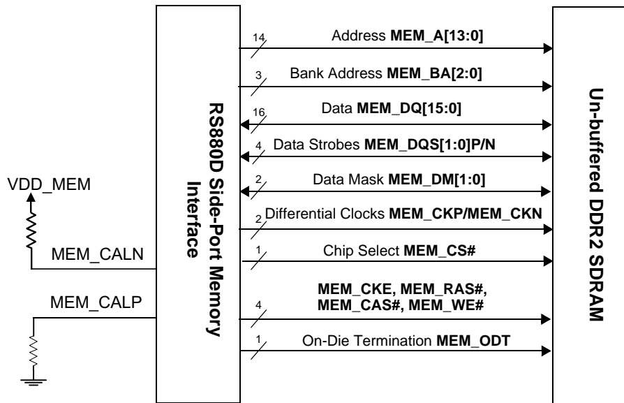
Figure 2-4 RS880D Side-Port Memory Interface
