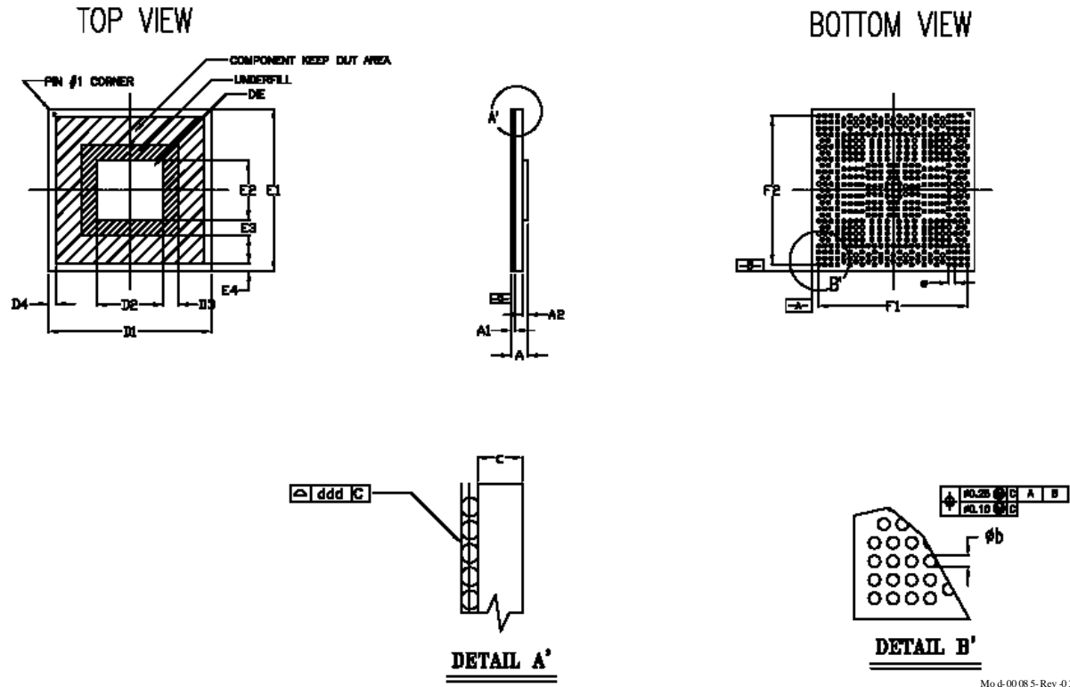
Figure 5-2 RS880D 528-Pin FCBGA Package Outline
