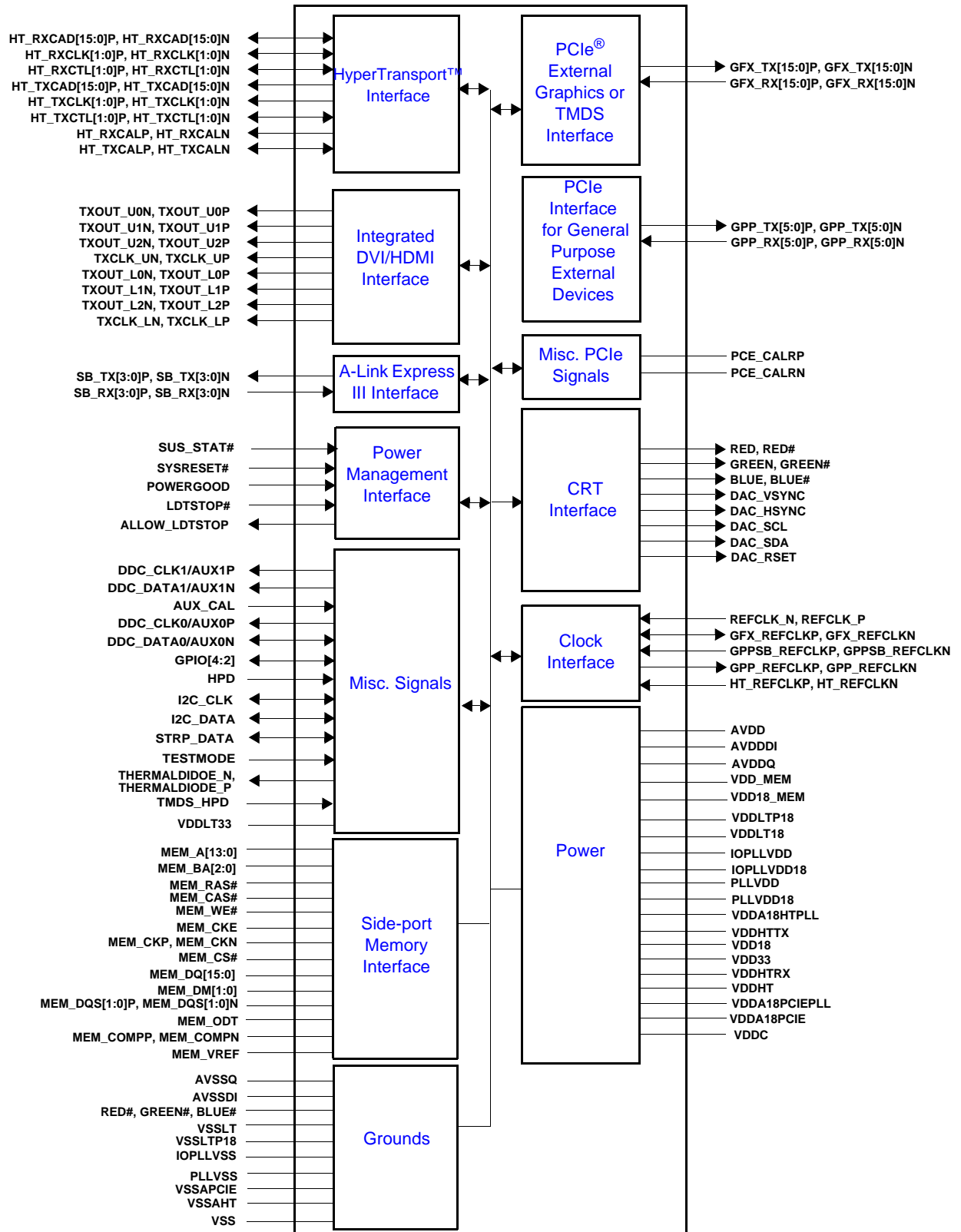
Figure 3-3 RS880D Interface Block Diagram
