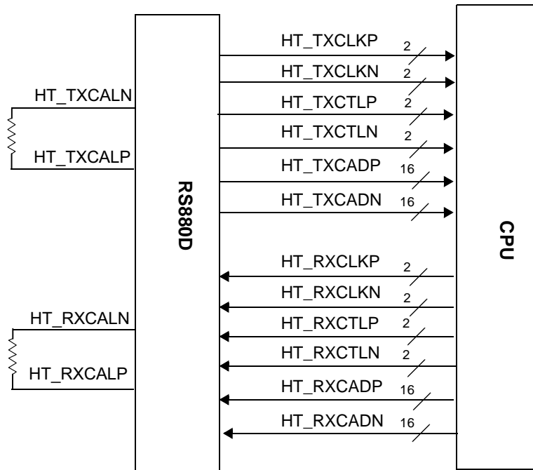
Figure 2-3 RS880D Host Bus Interface Signals
