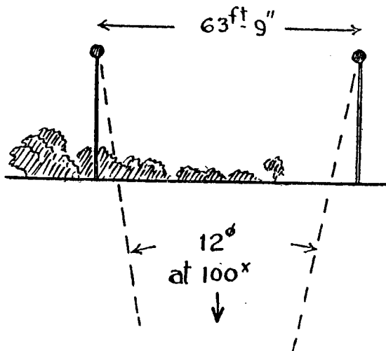
FIG. 9.—12-degree lead marks—sky background.
