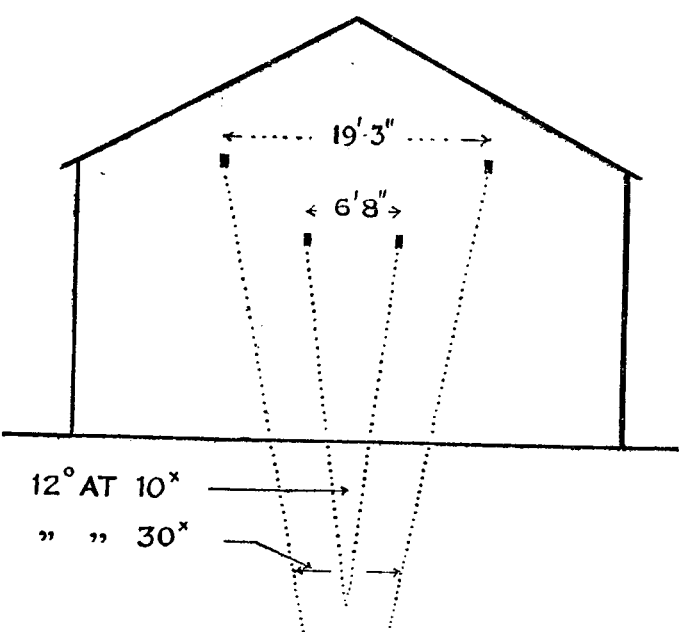
FIG. 8.—12-degree lead marks on wall of building.
