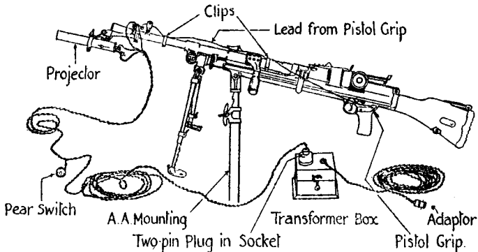
FIG. 14.—L.M.G. fitted with complete spotlight equipment.
