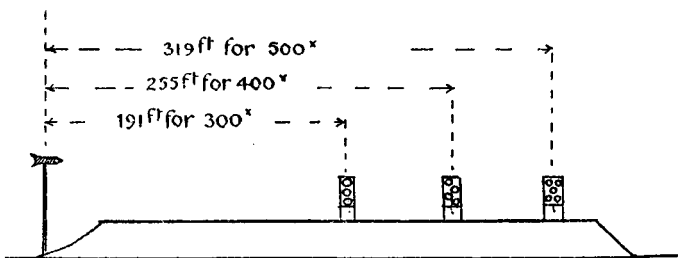
FIG. 10.—12-degree measurements on a rifle range.
