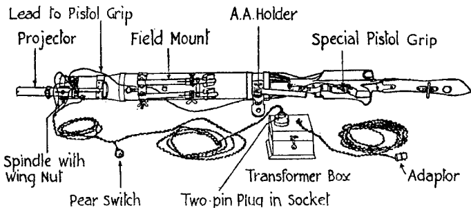
FIG. 16.—Lewis gun fitted with complete equipment.
