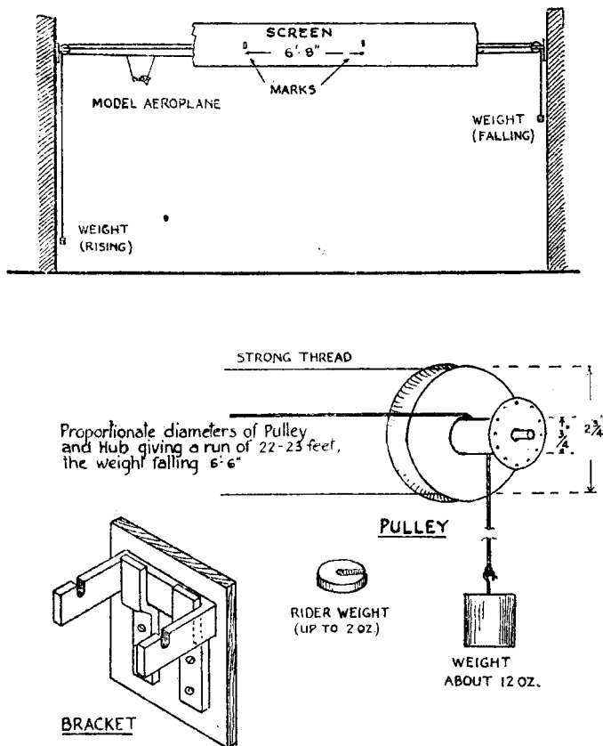
FIG. 18.—Moving target for spotlight projector.
