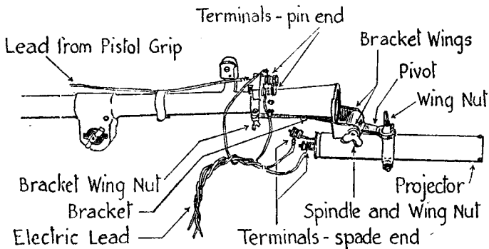
FIG. 15.—Projector fitted to muzzle of L.M.G.
