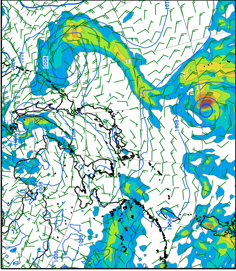
T=36 valid 241200UTC SURFACE PRESS(hPa), WIND(KNOTS) AT SURFACE PRECIP(MM)(24-36)
