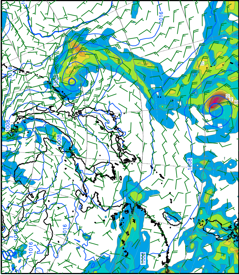
T=24 valid 240000UTC SURFACE PRESS(hPa), WIND(KNOTS) AT SURFACE WS_FXFE03 230000UTC May 2012
