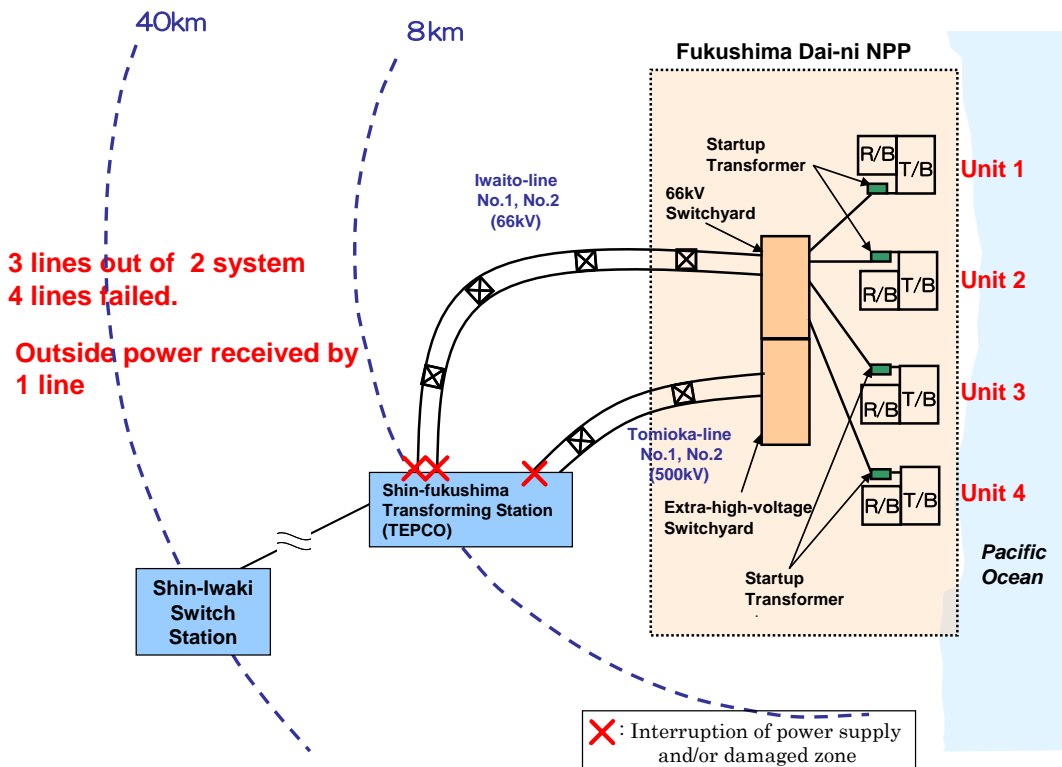
Fig. III-2-8(a) Damage of external power supply systems for the Fukushima Dai-ichi and Dai-ni NPSs (1).
